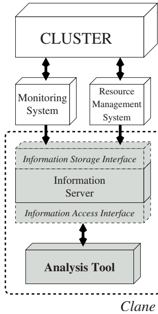
Fig. 2. Clane architecture
