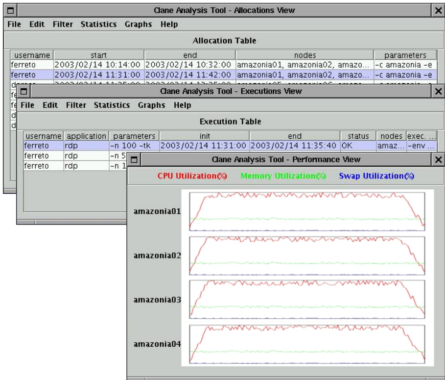
Fig. 3. Clane Analysis Tool
