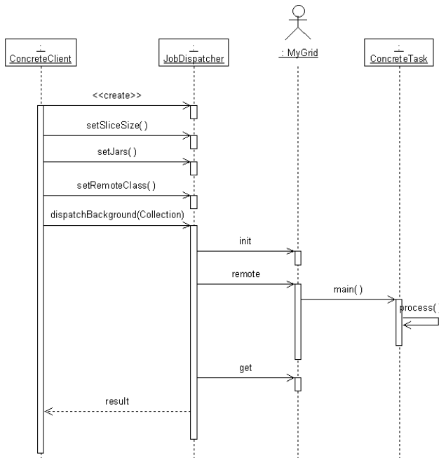
Figure 4. OJAL Sequence Diagram
