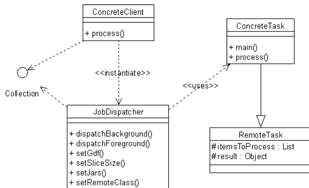
Figure 3. OJAL Class Diagram
