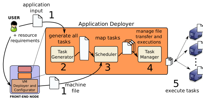
Fig. 4. Application deployer.
