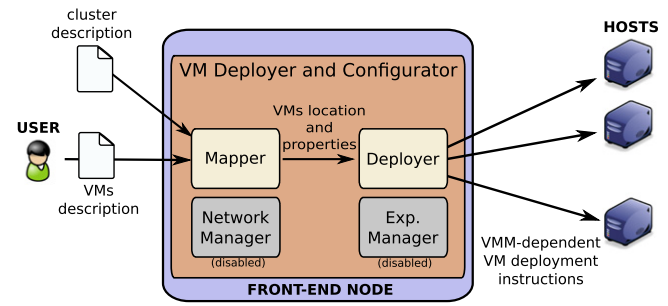
Fig. 5. AEF framework.
