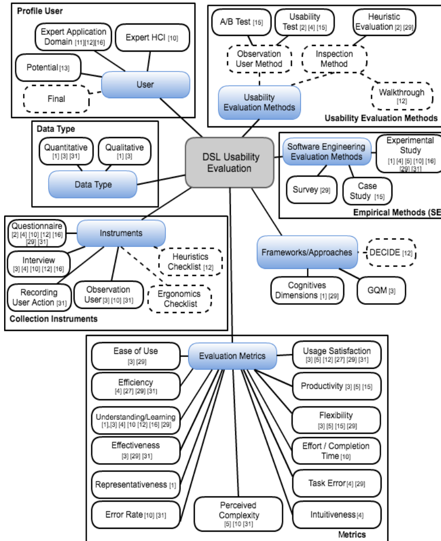
Fig. 3. DSL usability evaluation taxonomy
