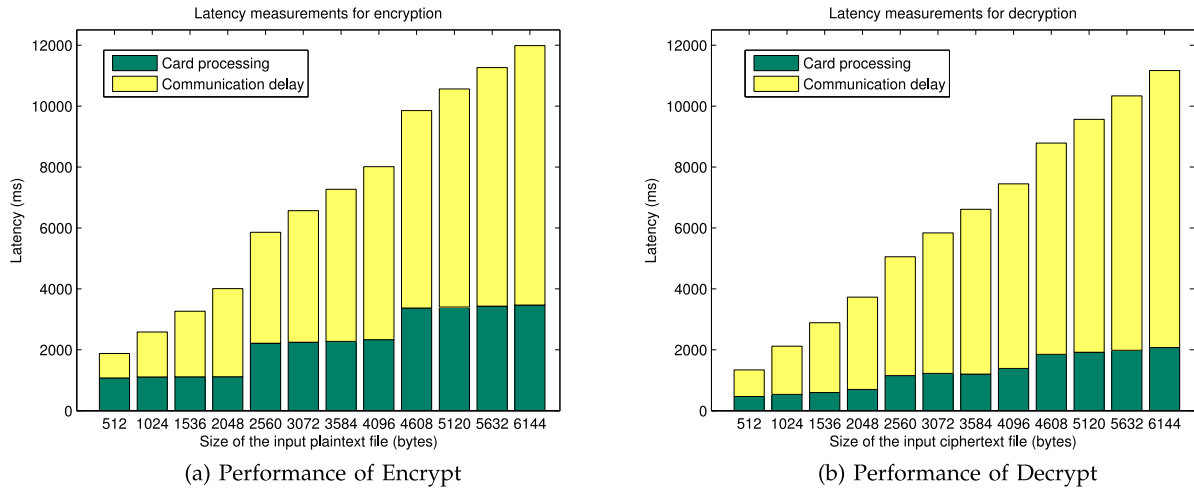
Fig. 4. Performance evaluation based on a proof-of-concept implementation using a resource-constrained Java card (5 MHz processor). The same implementation should work several hundred times faster on a high-performance Tamper Resistant Module such as IBM Storage Manager HSM (2 GHz processor) [43].
