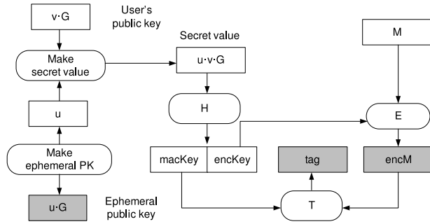
Fig. 1. Encrypting with DHIES [1]. The symmetric encryption algorithm is denoted as E , the MAC algorithm as T and the hash function as H . The shaded rectangles constitute the ciphertext.
