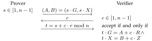
Fig. 2. Chaum-Pedersen protocol [9]: a zero-knowledge proof technique to prove the statement that (G, X, R, Z) = (G, x \cdot G, r \cdot G, x \cdot r \cdot G) is a DDH tuple.
