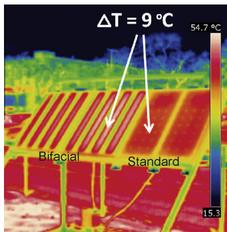
Fig. 7. Thermographic image of modules obtained in a cloudless day in spring.
