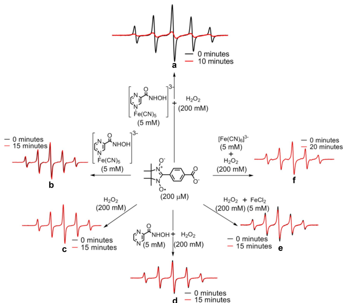
Fig. 4 a EPR signal of the cPTIO radical in the presence of the complex 3 under its protonated form 3\text{H}^+ and \text{H}_2\text{O}_2 ( t_0 =black line and t_{10\text{min}} =red line) in phosphate buffer solution, 40 mM, pH 7.4. b Control of the stability of the cPTIO EPR signal in the presence of \text{Na}_3[\text{Fe}(\text{CN})_5\text{-PyzCONHOH}] ( t_0 =black line and t_{15\text{min}} =red line). c Control of the stability of the cPTIO EPR signal in the presence of \text{H}_2\text{O}_2 ( t_0 =black line and t_{15\text{min}} =red line). d Control of the stability
