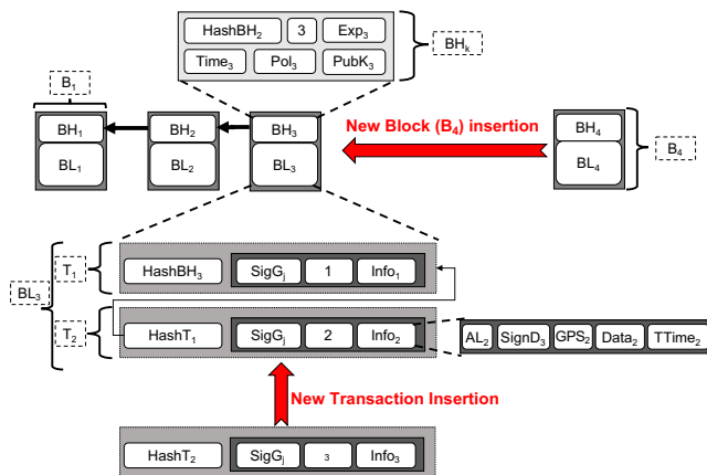
Fig. 1: Appendable-block blockchain block insertion and transaction insertion (adapted from [12]).
