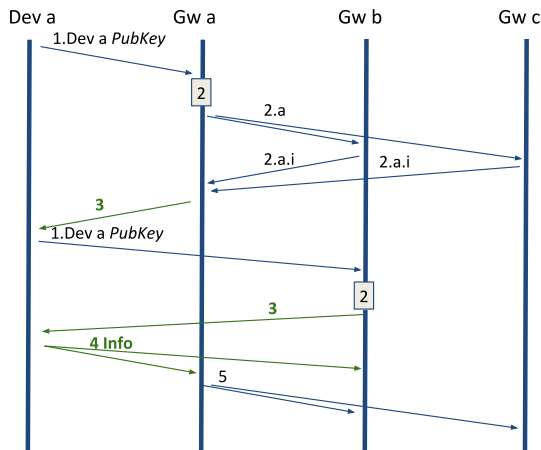
Fig. 2: Device connection simplified protocol.
