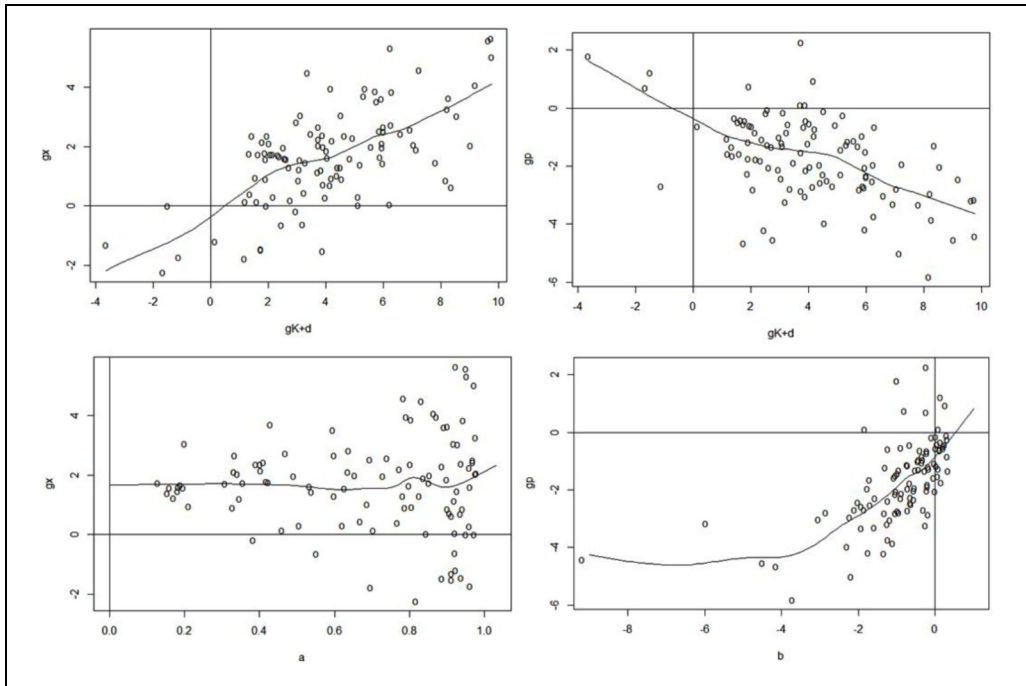
Figure 5. The relationships between capital accumulation and the growth rate of labor productivity, ( g_K + d, g_L ), between capital accumulation and the growth rate of capital productivity, ( g_K + d, g_P ), between the gap in labor productivity in 1980 and the growth rate of labor productivity, ( a, g_L ), and between the gap in capital productivity in 1980 and the growth rate of capital productivity, ( b, g_P ), 1980–2014.
