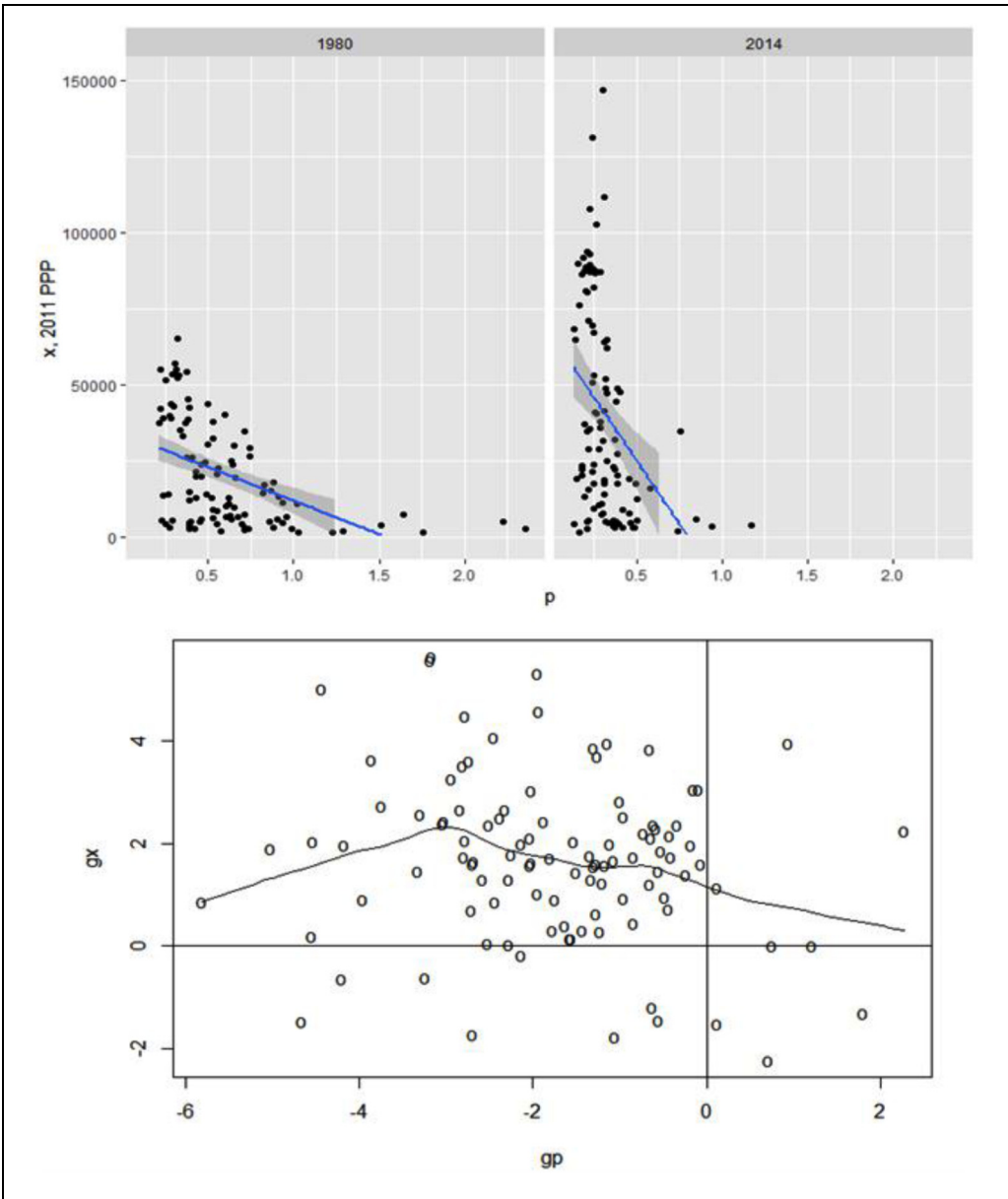
Figure 4. The capital and labor productivity points ( p, x ) and the compound growth rates of capital productivity and labor productivity ( g_p, g_x ) between 1980 and 2014. Source: See appendix I.
