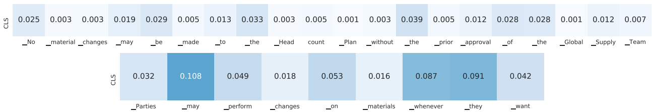
Figure 5.3 – Heat map with attention weights produced by NCC-Model nli-ft for the norm pair of the last row of Table 5.3, which contains a deontic-structure conflict.
