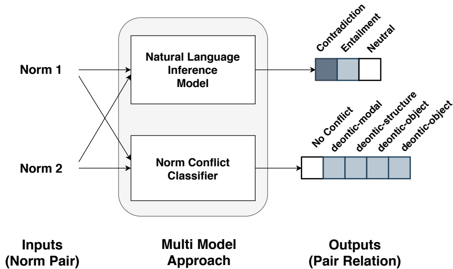
Figure 3.1 – Diagram illustrating our multi-model approach processing a norm pair, which results in two logit vector: one that represents the likelihood of the norm pair belonging to a particular conflict type conflict type (or nonconflicting) and another to represent its inferential relation (NLI classes).
