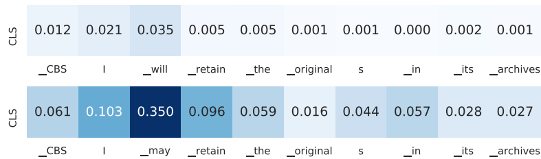
Figure 5.1 – Heat map with attention weights produced by NCC-Model_{nli-ft} for the norm pair of the first row of Table 5.3, which contains a deontic-modality conflict. Due to space limitations, we divide the self-attention vector in two rows to represent each sentence in a row and we omit the special characters.
