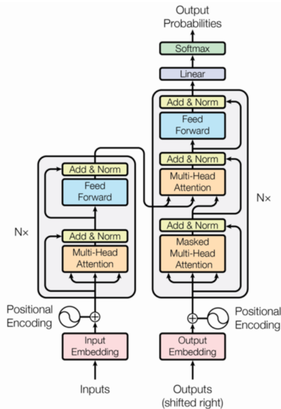
Figure 2.4 – Diagram of Transformer architecture describing the layer composition of blocks. [35]
