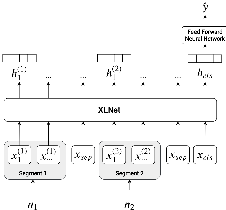
Figure 3.2 – Multi-label classifier that uses XLNet to generate tokens representation followed by a Feed Forward Neural Network to predict the output class.
