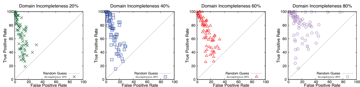
Figure 2: ROC space for all four percentage of domain incompleteness.
