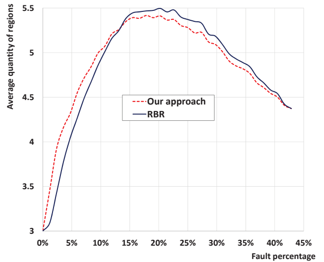
Fig. 3. Average quantity of regions according to the percentage of faults.
