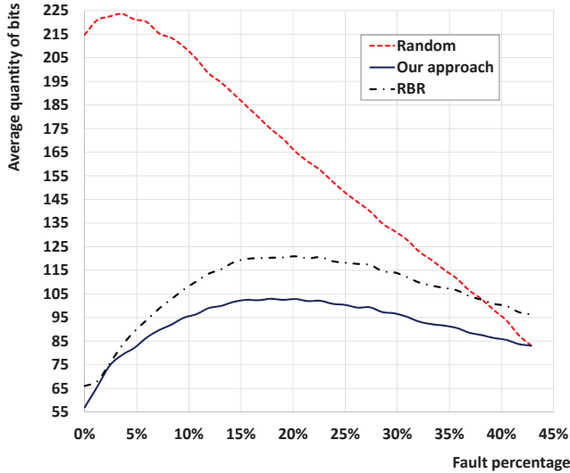
Fig. 5. Average quantity of bits required for each selection method according to the percentage of faulty links on NoC.
