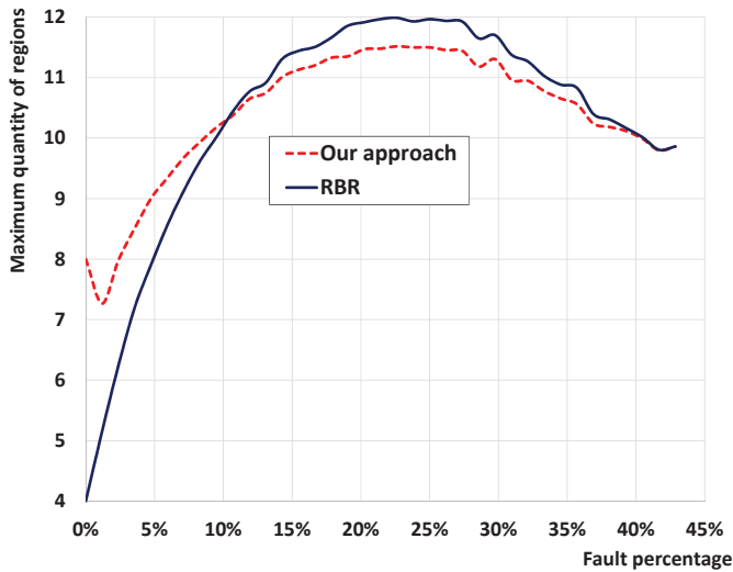
Fig. 2. Maximum quantity of regions regarding the percentage of faults.
