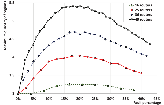
Fig. 6. Comparison of the maximum quantity of regions for four NoC sizes.
