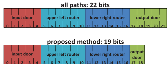
Fig. 4. Number of bits for storing a region.
