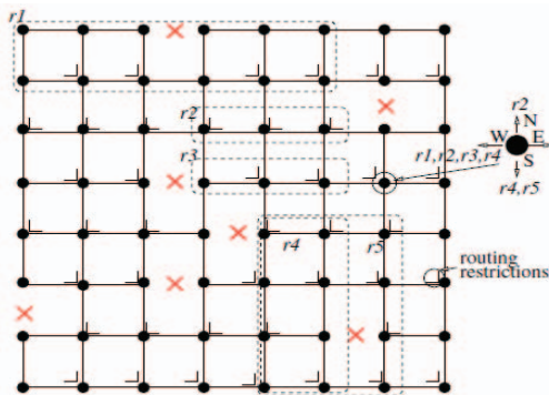
Fig. 1. An irregular 8x8 mesh NoC showing RBR applied to five regions [8].
