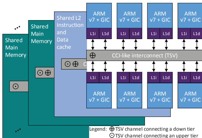
Figure 1. Target architecture comprising eight ARM-v7 processors in an SMP architecture. TSVs are used to connect memory models of other 3D tiers.
