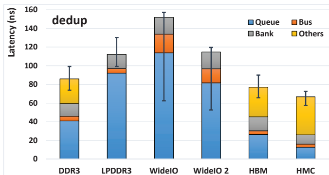
Figure 3. Average of DRAM and L2 latency for the Dedup application. Error bars represent the lowest and highest average values encountered.
