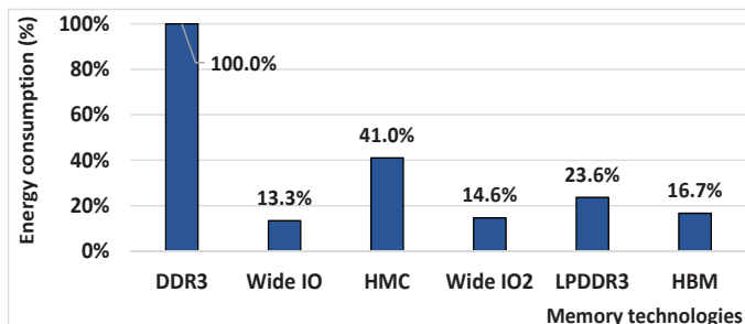
Figure 4. Average energy consumption of all evaluated memories during PARSEC execution.
