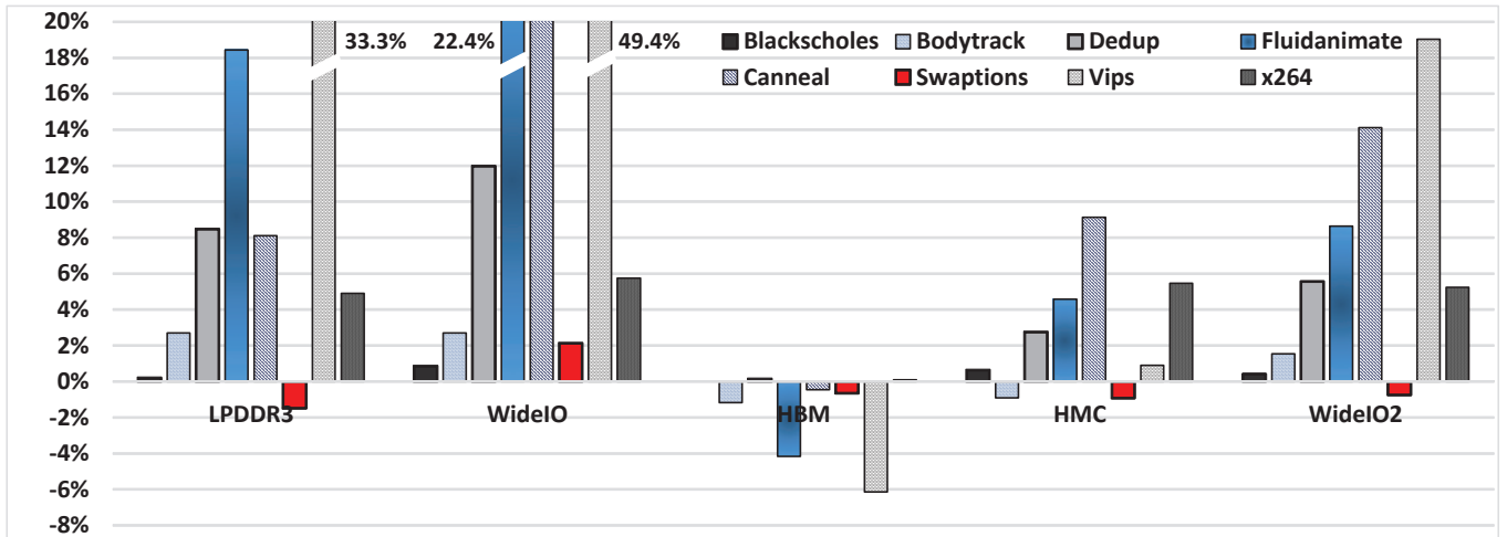
Figure 2. The execution time of eight applications versus six memory technologies. All values are relatively normalized according to the DDR3; i.e., for all applications, the execution time of DDR3 is 0% and the remaining values are perceptual deviations of this reference.
