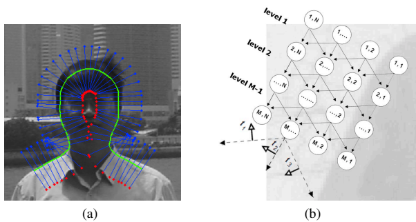
Fig. 6. Illustration of the graph. (a) The green line represents the generated skeleton curve S_{s,j} for a specific cluster j , whilst the blue lines illustrates the levels of the graph; (b) a detailed illustration of the graph, with its nodes and edges.
