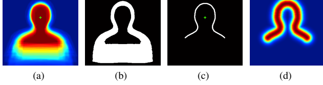
Fig. 4. Shape model generation. (a) Initial shape model S_{0,j} and the reference point R_{p,j} ; (b) thresholded image; (c) skeleton image S_{s,j} and (d) final shape mask S_{f,j} for a given class j .
