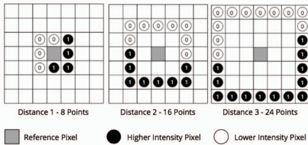
Figure 6 – LBP Matrices
