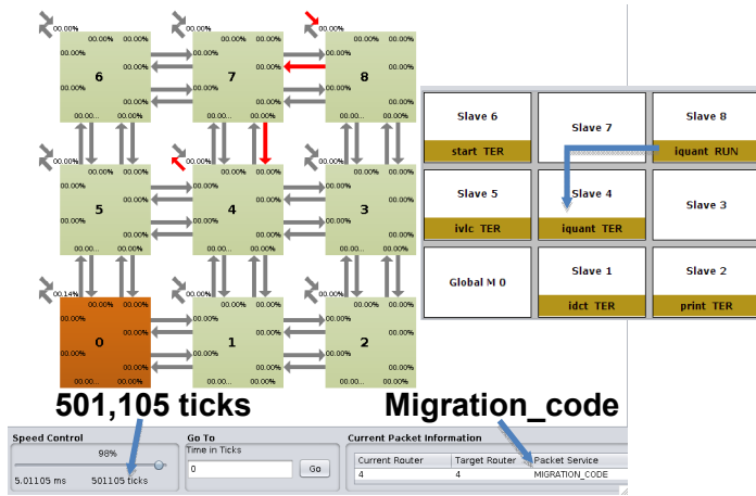
Figure 6 – Debug process for task migration protocol, with task iquant (MJPEG application) migrated from PE 8 to PE 4.
