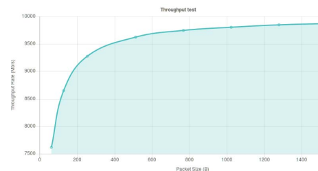
Fig. 4: Throughput test results.
