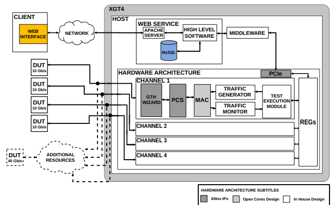
Fig. 1: The XGT4 system architecture block diagram.
