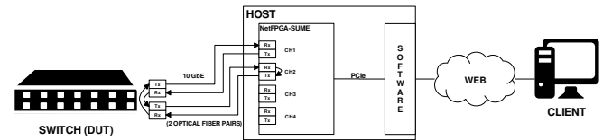
Fig. 3: XGT4 validation setup.
