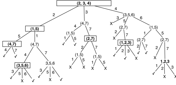
Fig. 3. Computing all justifications using Reiter's Hitting Set Tree Algorithm from
