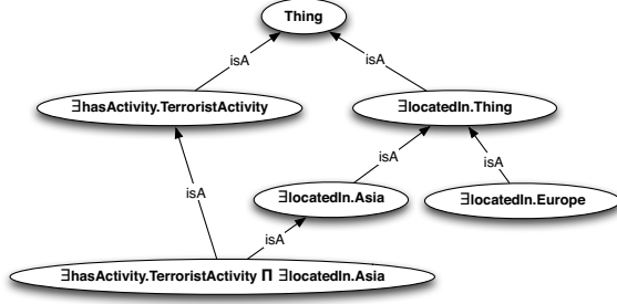
Fig. 2. Context hierarchy
