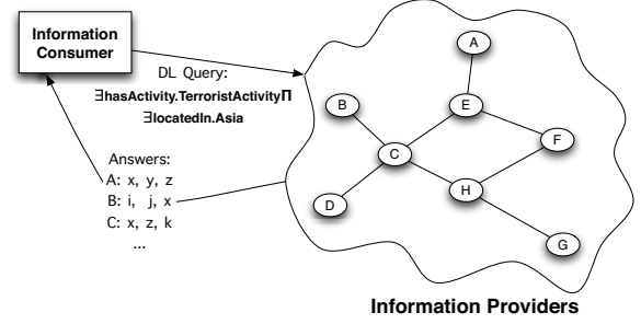
Fig. 1. A simple scenario demonstrating the interactions between consumers and providers
