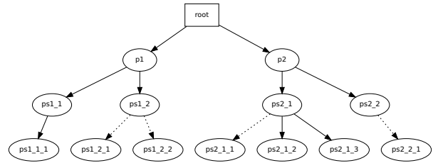
Fig. 1. Example of a plan library tree created by the Plan Library Generator with np = 2 , dt = 3 , mi = 1 , ma = 3 , sq = 0.5 , fs = 3 , fn = 1 , mv = 2 , and pd = 0 .
