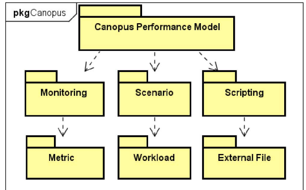
Figure 2: Canopus class diagram
