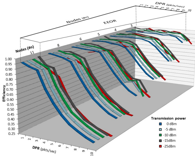
Figure 1. Relation between efficiency and data rate for some number of nodes and transmission power values. Additionally, a polygon representing a perspective of linearization of EEOR.
