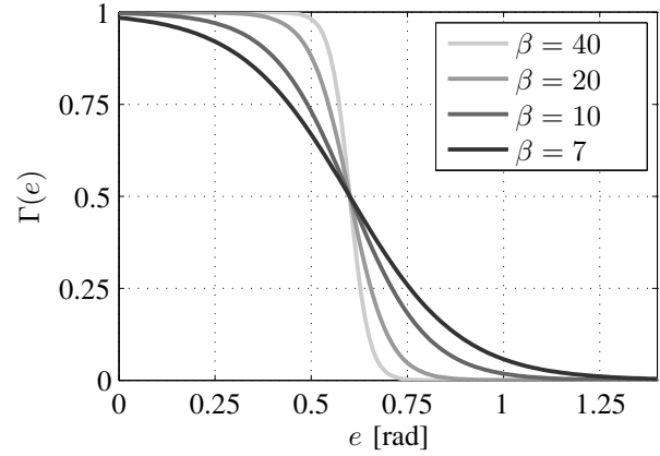
Fig. 6: Function \Gamma(e) in (10) for different values of \beta .
