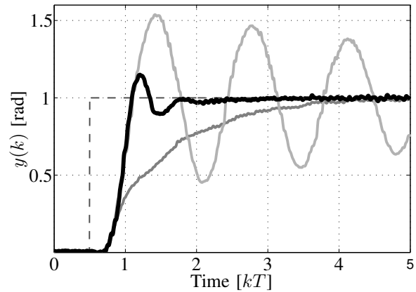
Fig. 7: System response to the different control laws from the origin to r = 1 rad. Legend: black line - proposed controller; light grey line - undamped controller; dark grey line - damped controller.
